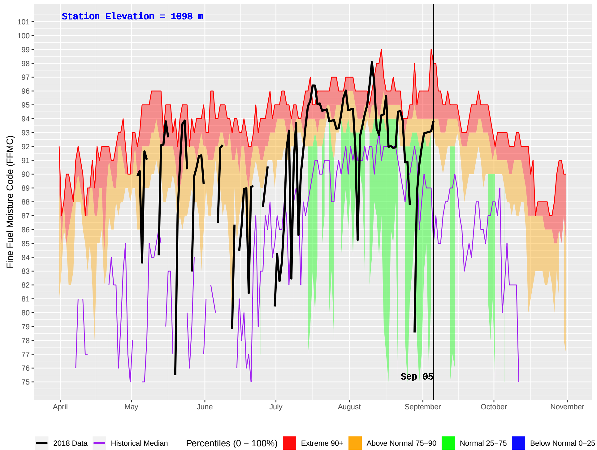
GOATFELL (401) : Historical (1986–2016) and Current (2018) Daily Fine Fuel Moisture Code (FFMC)
