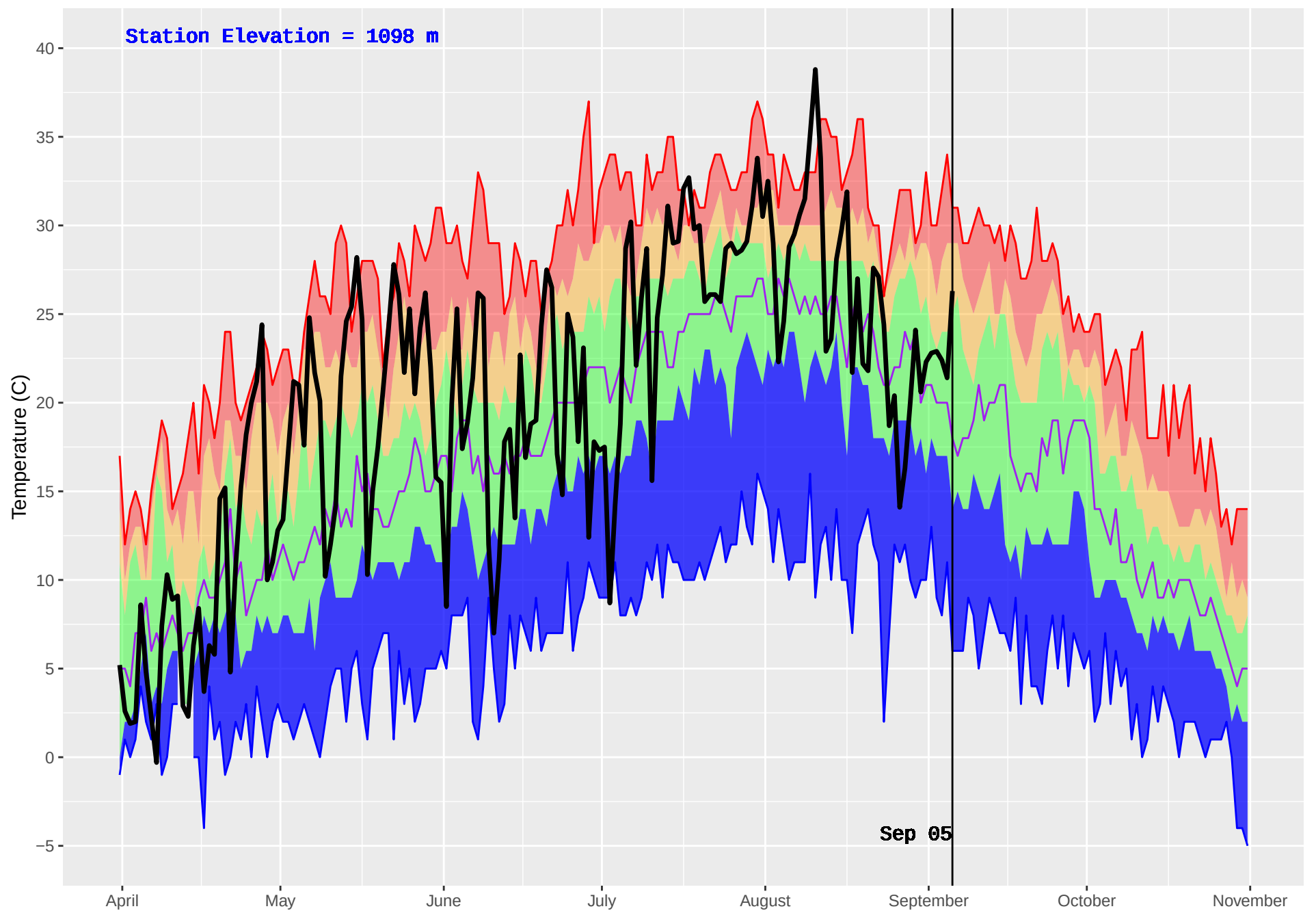
GOATFELL (401) : Historical (1986–2016) and Current (2018) Daily Temperature
