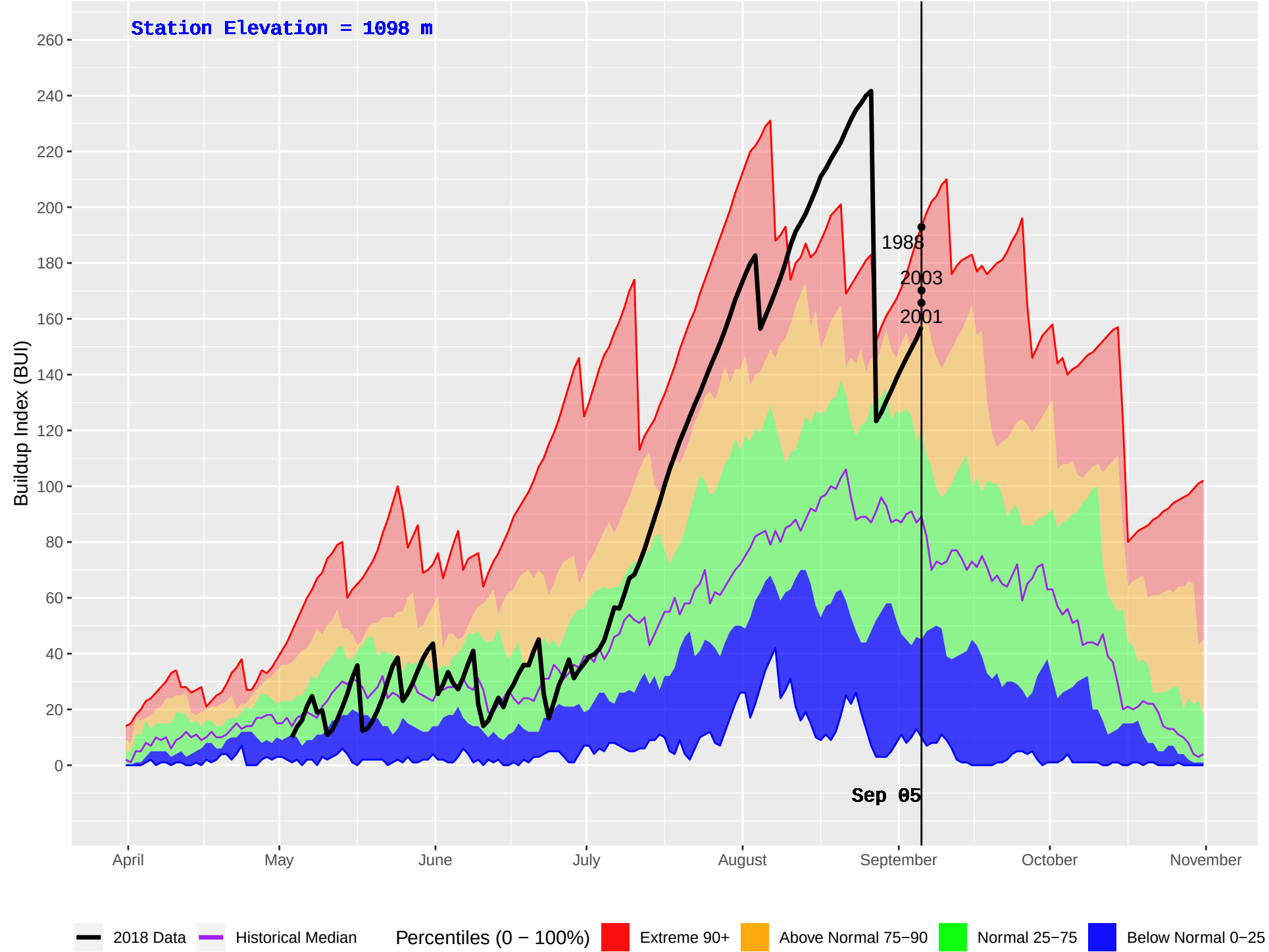
GOATFELL (401) : Historical (1986–2016) and Current (2018) Daily Buildup Index (BUI)
