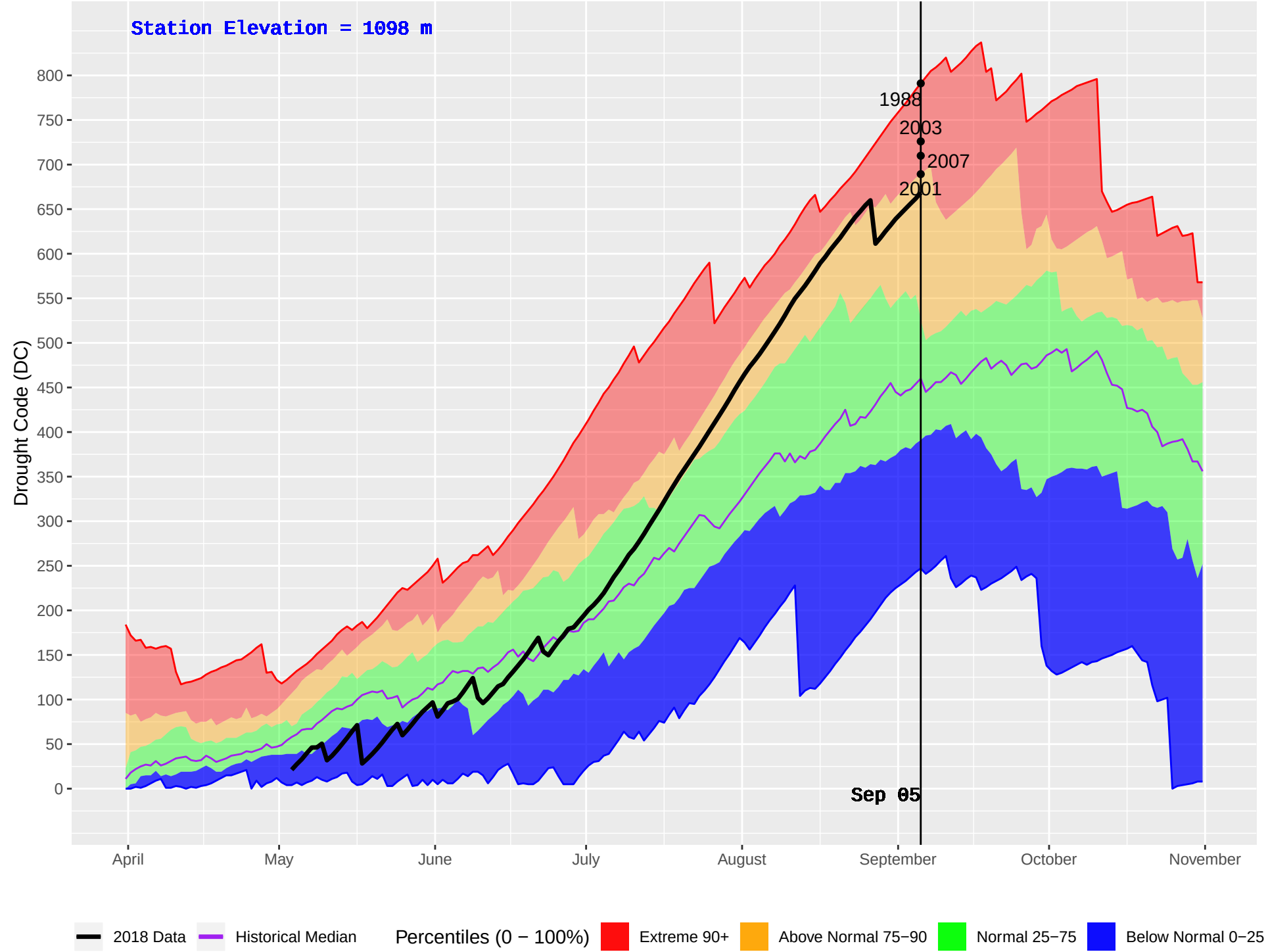
GOATFELL (401) : Historical (1986–2016) and Current (2018) Daily Drought Code (DC)
