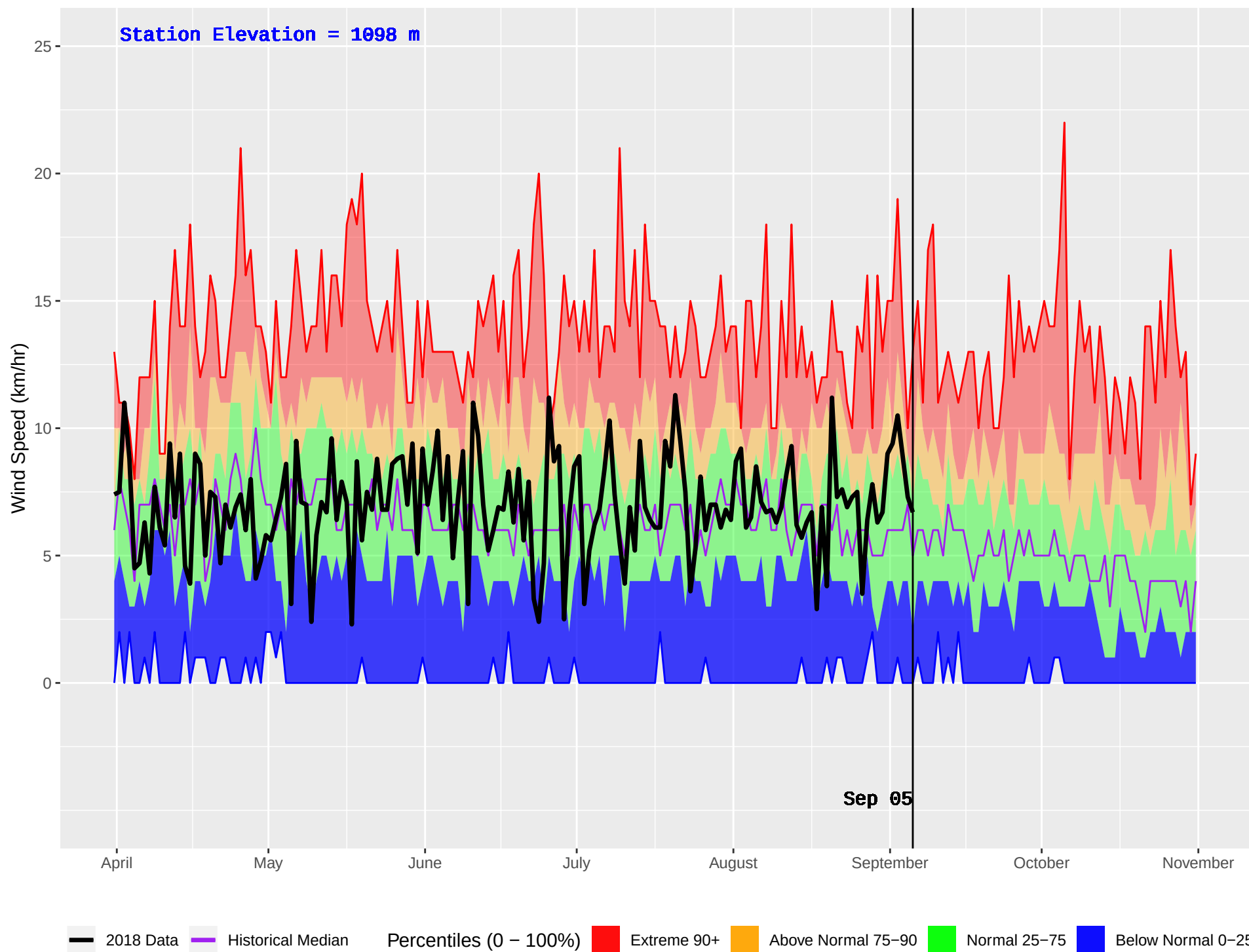
GOATFELL (401) : Historical (1986–2016) and Current (2018) Daily Wind Speed
