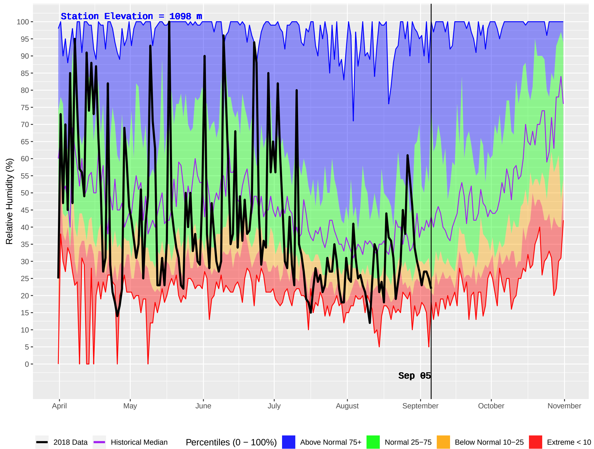
GOATFELL (401) : Historical (1986–2016) and Current (2018) Daily Relative Humidity
